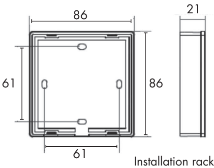
Installation rack
