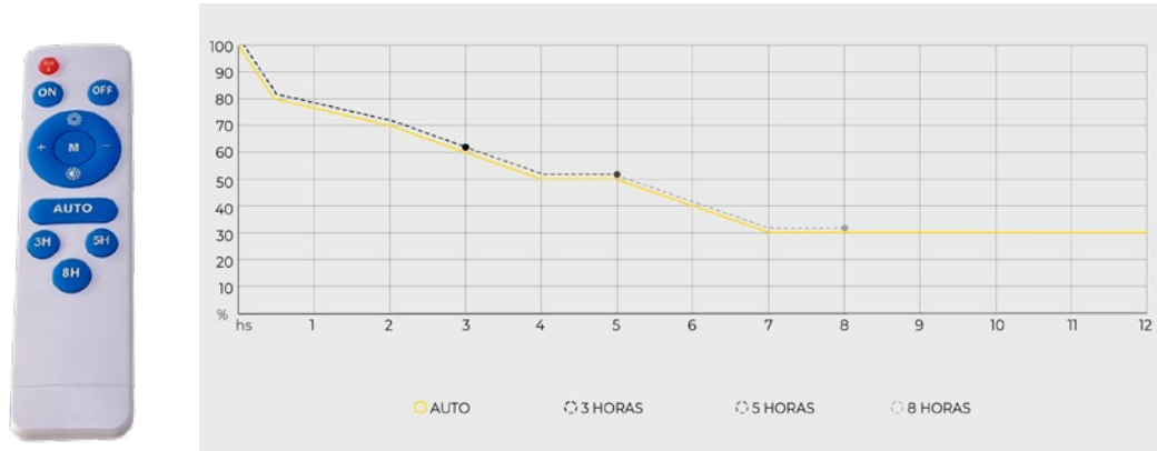
BRILLO DE LA LUMINARIA SOLAR - BRIGHTNESS OF SOLAR FLOOD LIGHT
